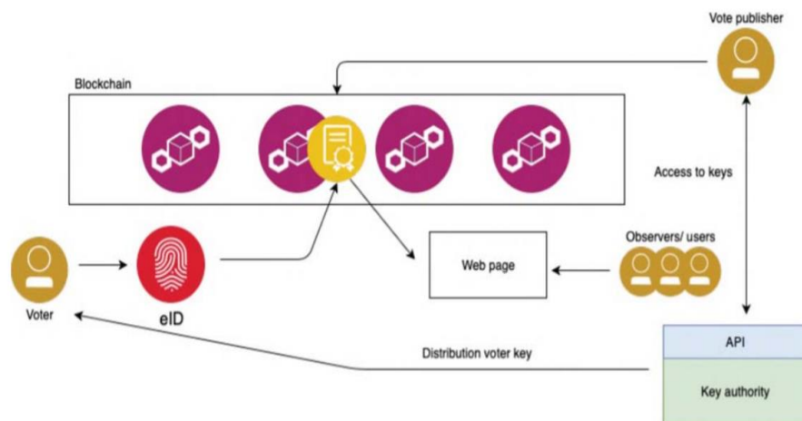
Fig. 1. High-Level architecture
